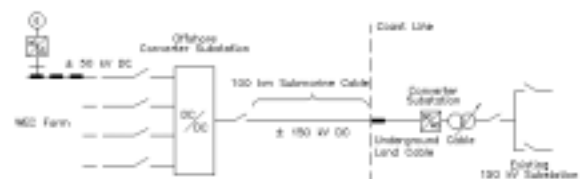
Figure 9 Transmission line - 100 km offshore (7)
