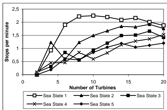
Figure 10 Turbine stops per minute as a function of number of installed turbines (9)
