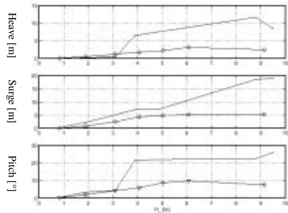
Figure 2 Heave, surge, and pitch before and after modifications to scale 1:50 model (26)
