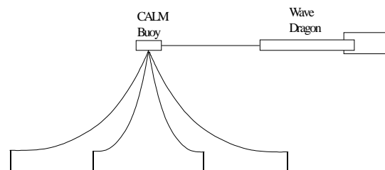
Figure 11 Example of a CALM buoy mooring system for the Wave Dragon (2)
