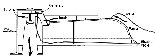
Cross section of the basin part
