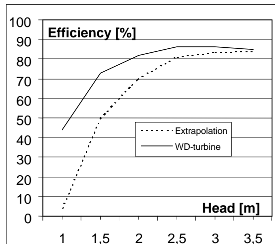
Figure 7 Fixed speed on/off Kaplan turbine w. cylinder gate inlet - expected vs. measured turbine performance, incl. intake & outlet losses
