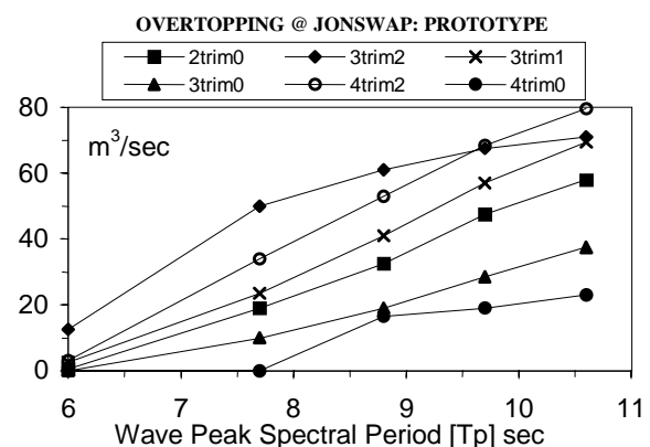
Figure 3 The effect of trim on performance in 1 - 5 m H_s long crested waves (30). 'XtrimY' means that the freeboard of the stern is X m, and the bow is lowered by Y m.
