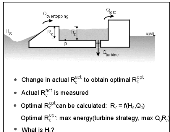
Figure 4 Regulation set-up
