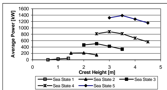
Figure 5 Average power as function of the freeboard crest height at different sea states. The figures are inclusive losses in the power train (14)
