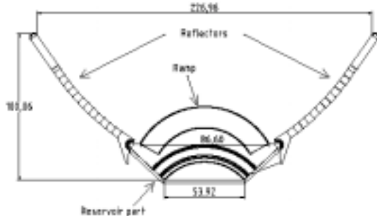
Figure 1 The Basic principle of the Wave Dragon
